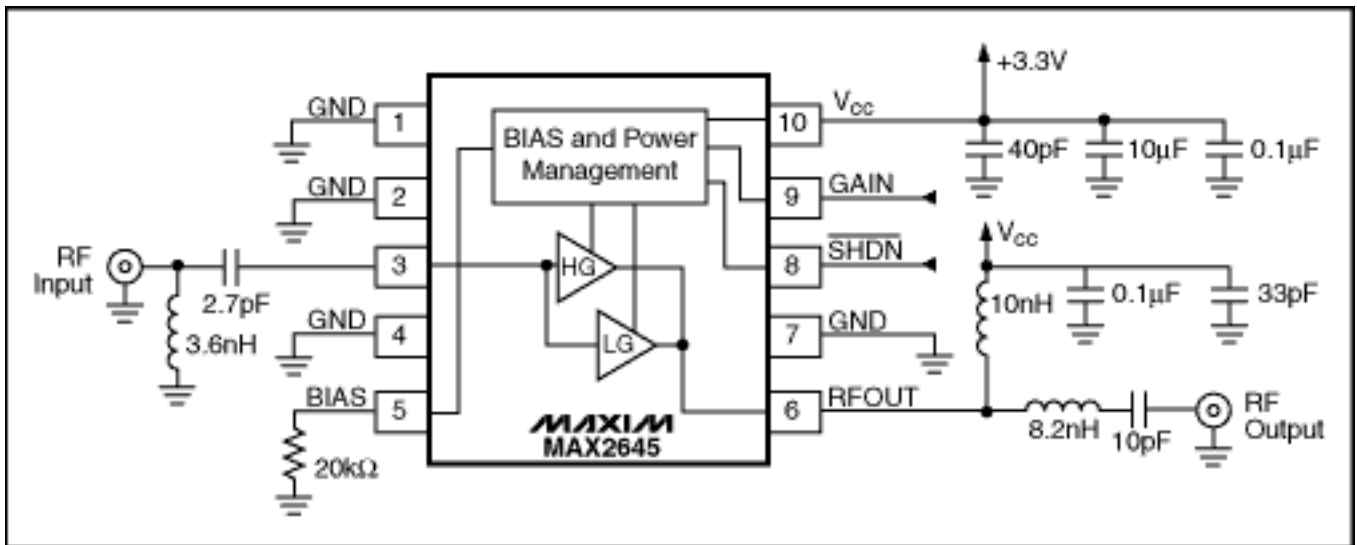
Figure 1. MAX2645 SiGe LNA Operating Circuit Optimized for 2.14GHz.
