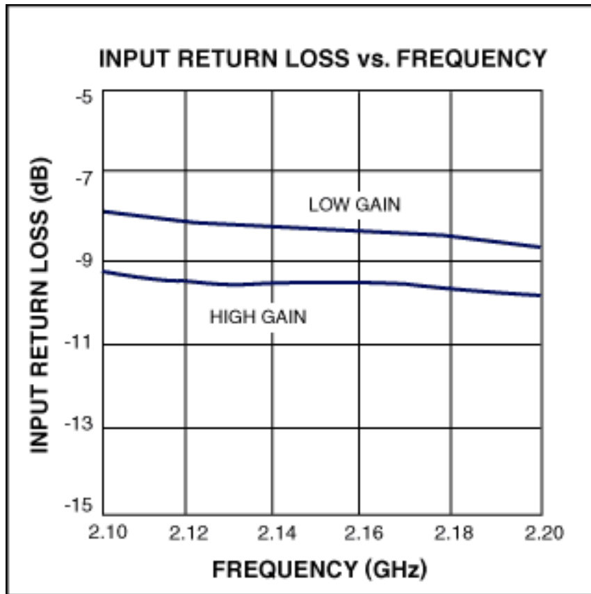
Figure 5. MAX2645 Input Return Loss vs. Frequency Plot.
