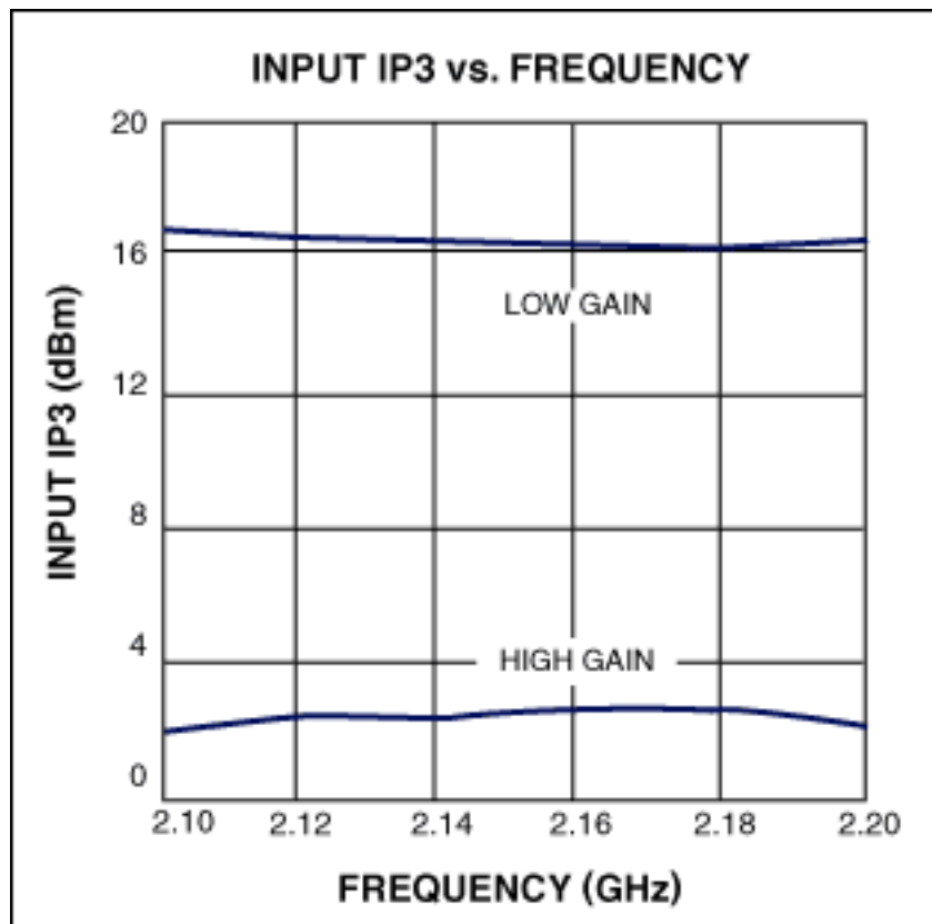
Figure 4. MAX2645 Input IP3 vs. Frequency Plot.
