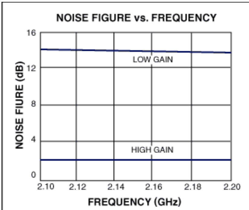
Figure 3. MAX2645 Noise Figure vs. Frequency Plot.
