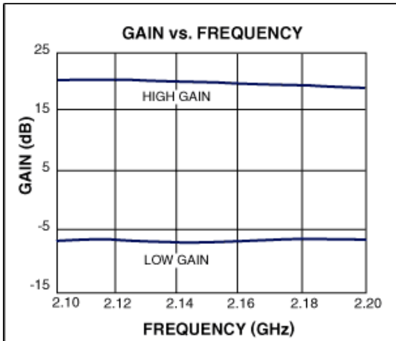
Figure 2. MAX2645 Gain vs. Frequency Plot.
